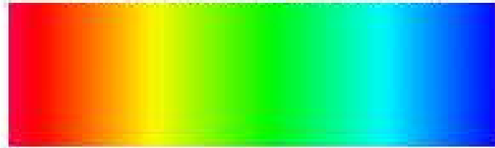
Continuum Spectrum
